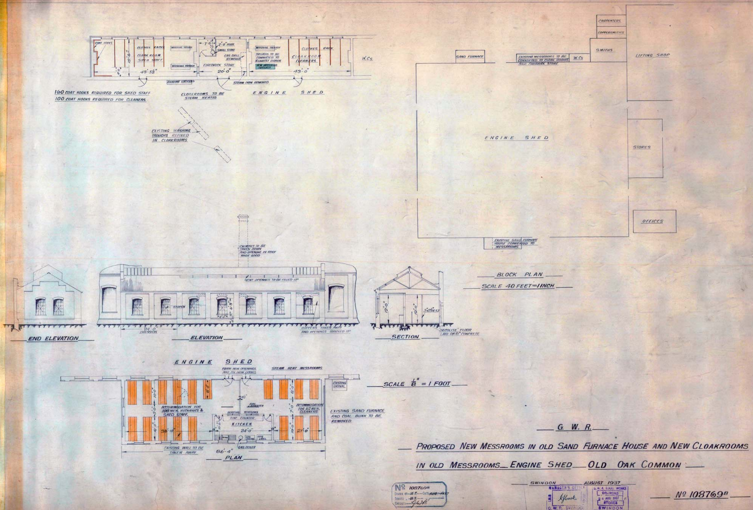
Figure 20.1: Plans from conversion of sand furnace in 1937
