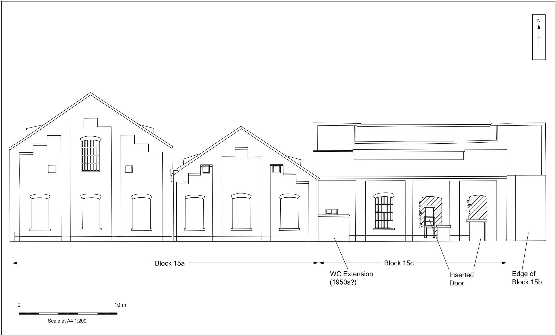
Figure 15a.2: Building 15. North Elevation
