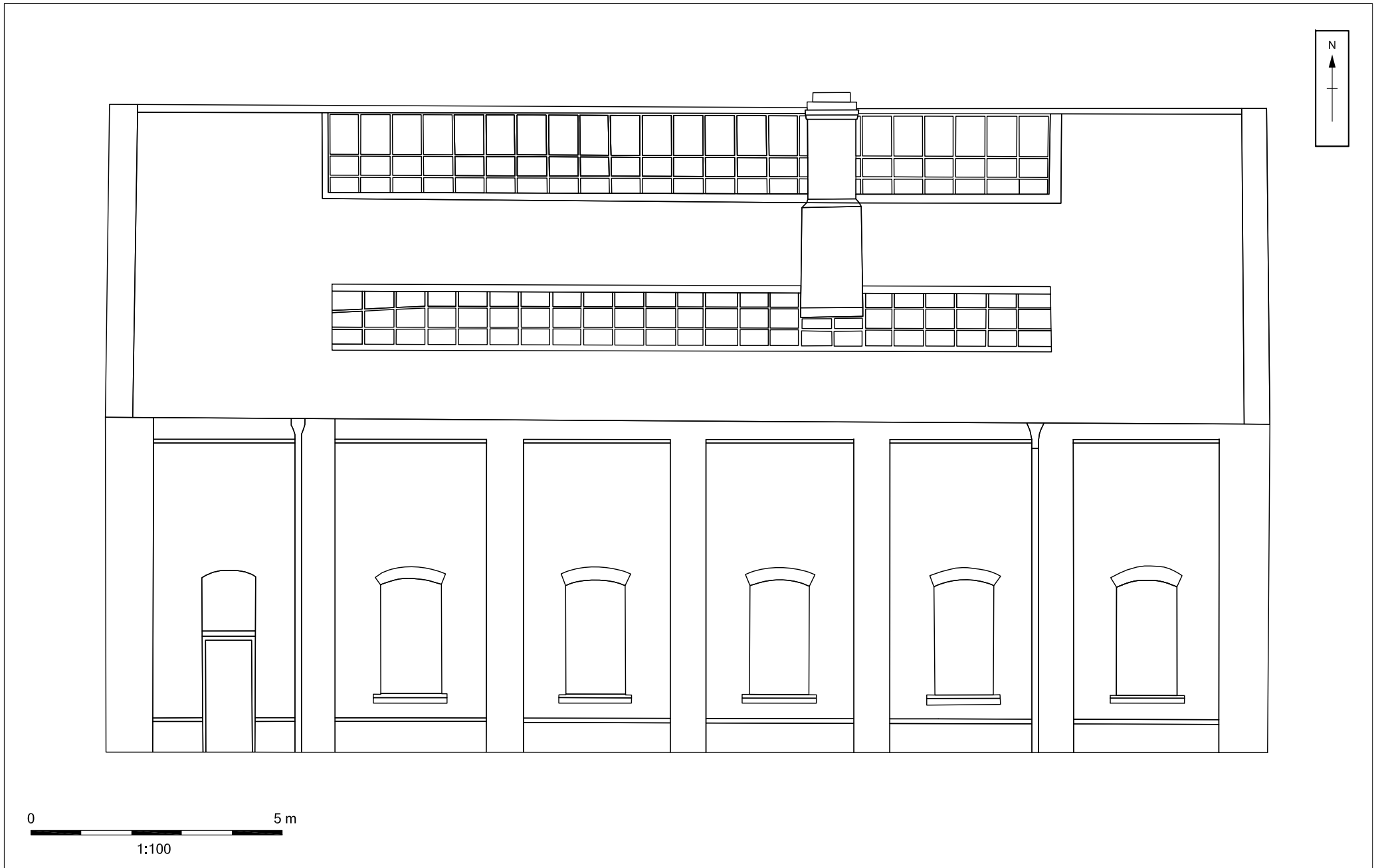
Figure 16.4: North Elevation, Building 16
