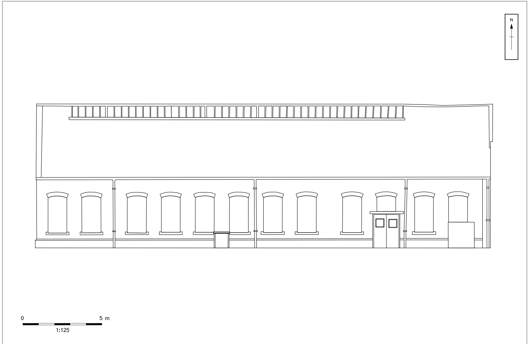
Figure 17a.4: Building 17a, South facing elevation
